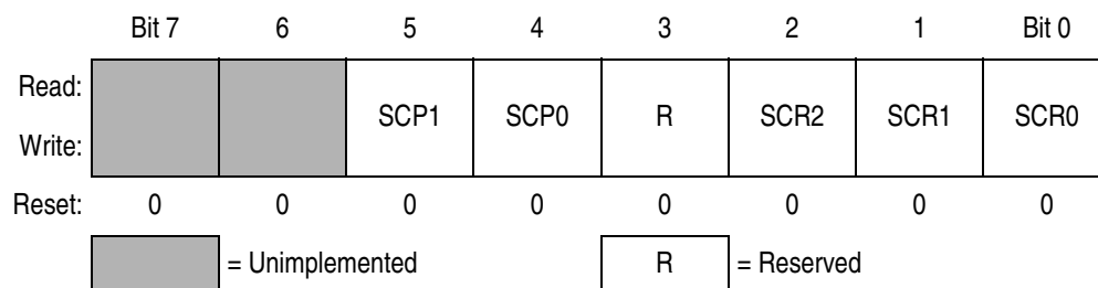
Figure 18-16. SCI Baud Rate Register (SCBR)
