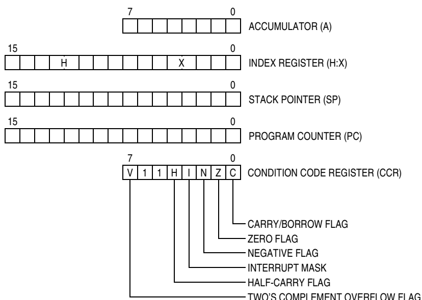
Figure 10-1. CPU Registers
